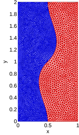
FIG. 5.4. Domains \Omega_1 (left) and \Omega_2 (right)
