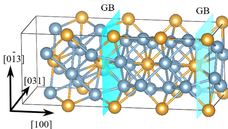
Fig. 1. Schematic presentation of the face-centred cubic Al \Sigma 5 [100] 36.87° twist grain boundary supercell. Both grain boundaries in the cell have been highlighted, along with the (yellow) atoms of the coincidence site lattice substructure to which the cell periodicity makes reference. The basis vectors for this substructure are expressed in units of the basis vectors for the central grain.
