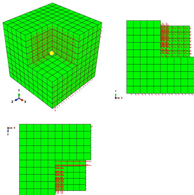
Figure 4.12. Visualization of the hydrogen flux \varphi ( \sim\varphi_d ). It can be observed that, as expected, this flux is collinear to m^g , in the (XY) plane. The yellow dot represents the central node.
