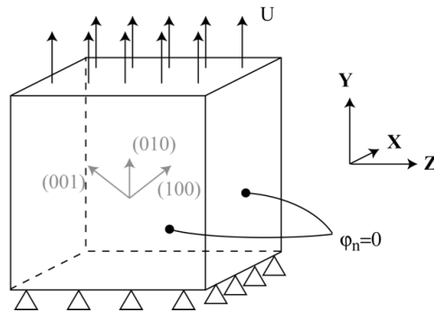
Figure 4.10. Single crystal configuration. (XYZ) denotes the global orthonormal coordinate systems. Displacement is applied along the Y direction.
