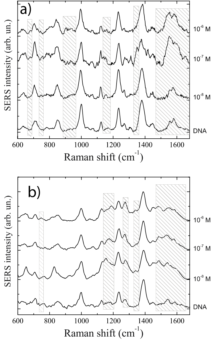
Figure 4: SERS detection of MnSOD at concentrations of 10 -6 , 10 -7 , 10 -8 M using (a) functionalized nanorods dimers (λ exc =785 nm) and (b) functionalized nanocylinders with 140nm diameter (λ exc =660 nm). For each SERS substrate the reference SERS spectrum of the functionalization layer is also shown (DNA). The dashed boxes highlight the spectral zones in which the protein provides strongest contribution. The spectra are plotted after background subtraction and offset vertically for clarity.
