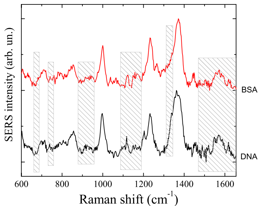
Figure 5: Negative control experiment. The SERS spectrum on gold nanorods dimers ( \lambda_{\text{exc}}=785\text{ nm} ) after incubation with BSA 10^{-5}\text{ M} (red line) does not show specific differences with respect to the SERS from the aptamer+MOH layer (black line) in the spectral zones in which the proteins feature their vibrational signal (dashed boxes). Spectra are offset vertically for clarity reasons.
