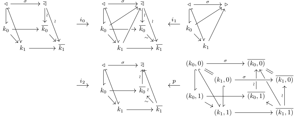
Figure 3: Zigzag diagram (45) for K = \{k_0 \rightarrow k_1\} \cong \Delta^1
