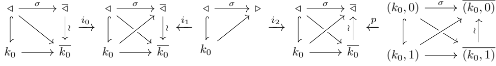
Figure 2: Zigzag diagram (45) for K = \{k_0\} \cong \Delta^0
