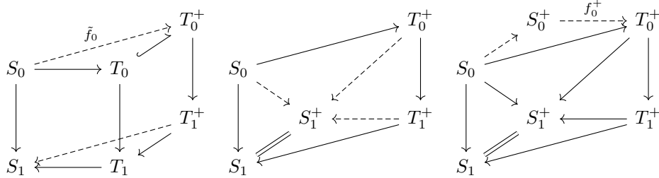
Figure 1: Diagrams of steps 1, 2 and 3 of the construction of f^+ . An arrow is dashed if it is added at the current step.
